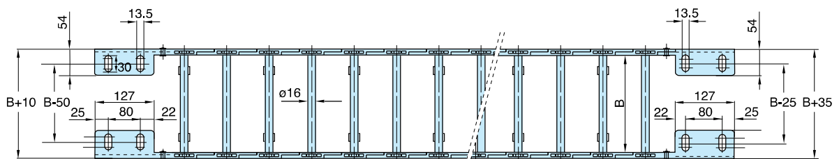
Fixed Bracket
