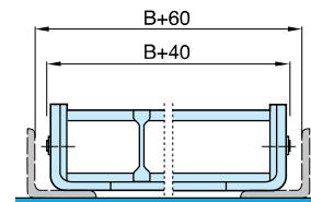
Guide Rail
