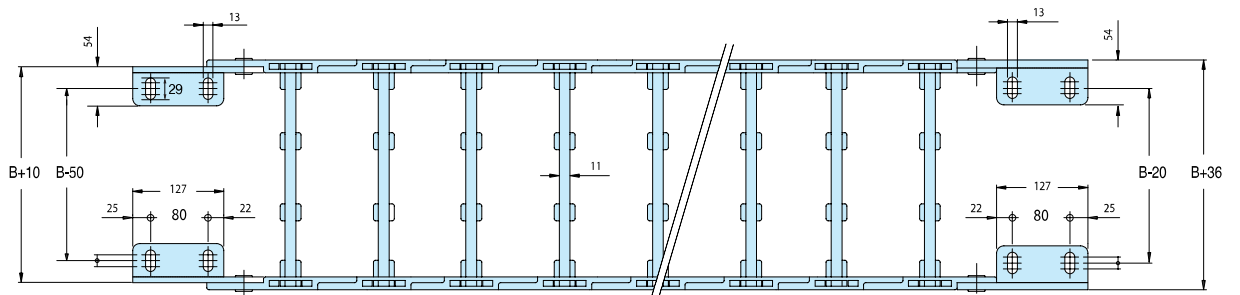
Fixed Bracket
