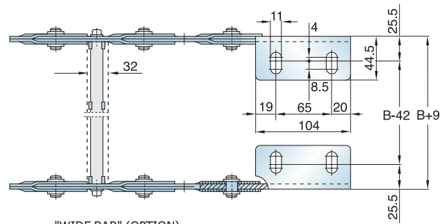
Moving Bracket
