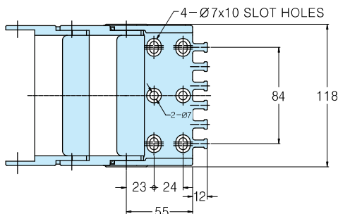
Fixed Bracket
