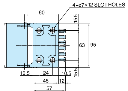
Moving Bracket
