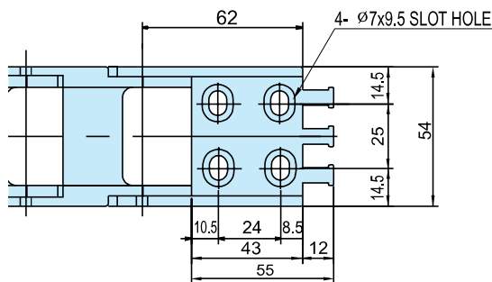
Fixed Bracket
