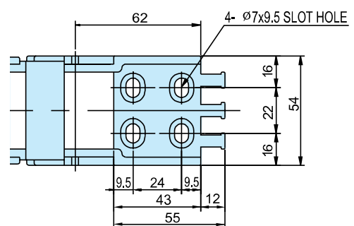
Moving Bracket
