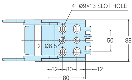
Fixed Bracket
