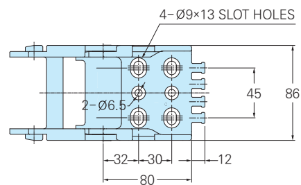
Moving Bracket
