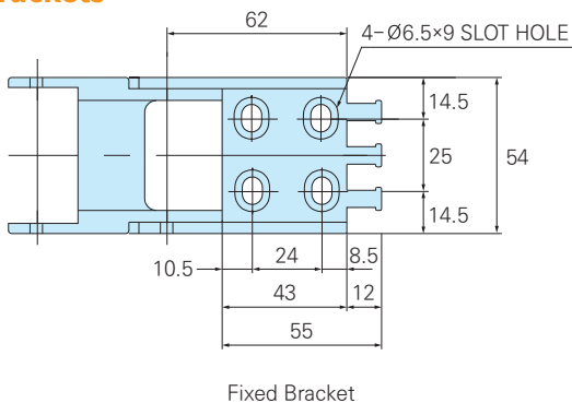
Fixed Bracket
