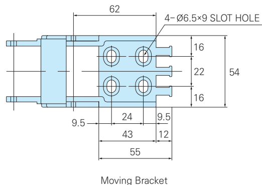
Moving Bracket
