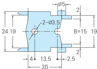
Moving-Fixed Link
