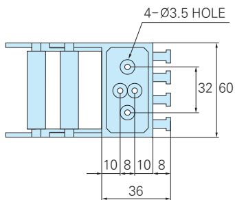
Fixed Bracket
