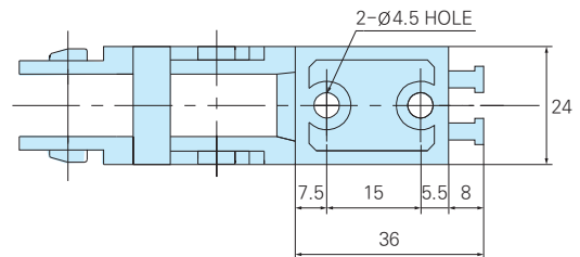
Moving Bracket
