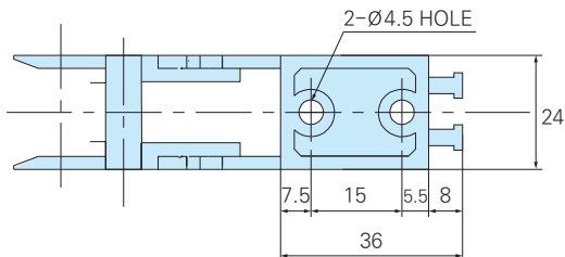
Fixed Bracket
