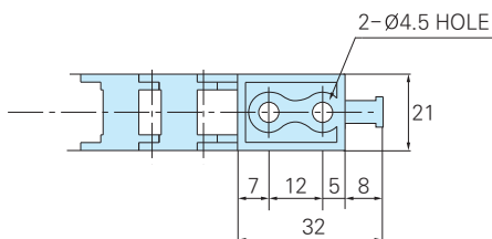
Fixed Bracket
