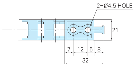
Fixed Bracket
