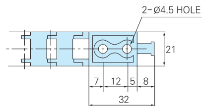
Moving Bracket
